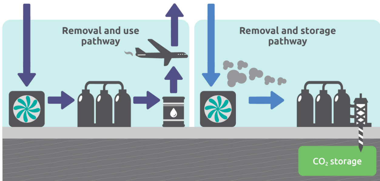
Figure 4.3 Example of carbon fluxes in a removals and use versus removals and storage pathway
