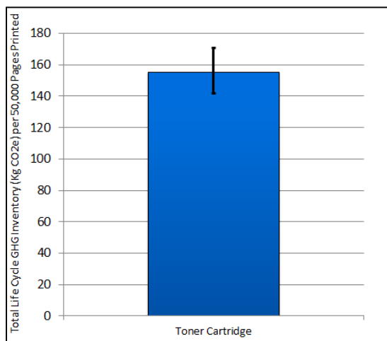
Figure [2] Impact assessment results of toner cartridge GHG inventory study
