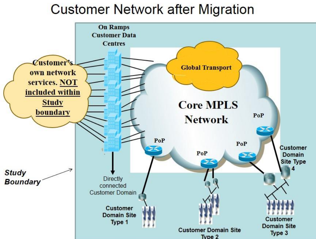
Figure A2.5. The boundary for the MPLS network service being studied
