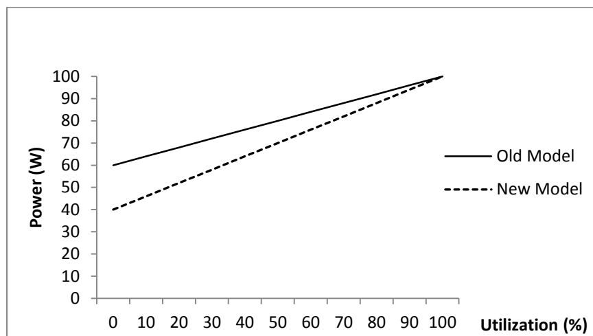
Figure 6.9. Correlation between server host resource utilization and power consumption
