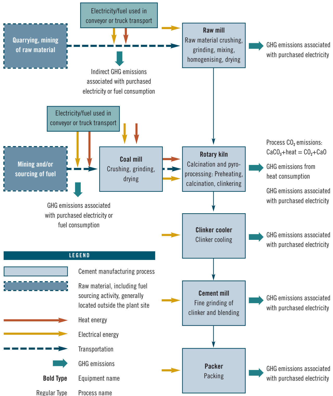
FIGURE E1.1 Flow diagram of cement manufacturing process (dry process with rotary kiln), with energy consumption points and types of GHG emissions generated in a cement facility
