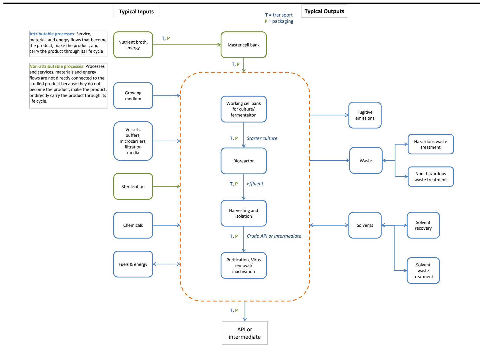
Figure 4.3 Sample Process Map for Cell Culture API
