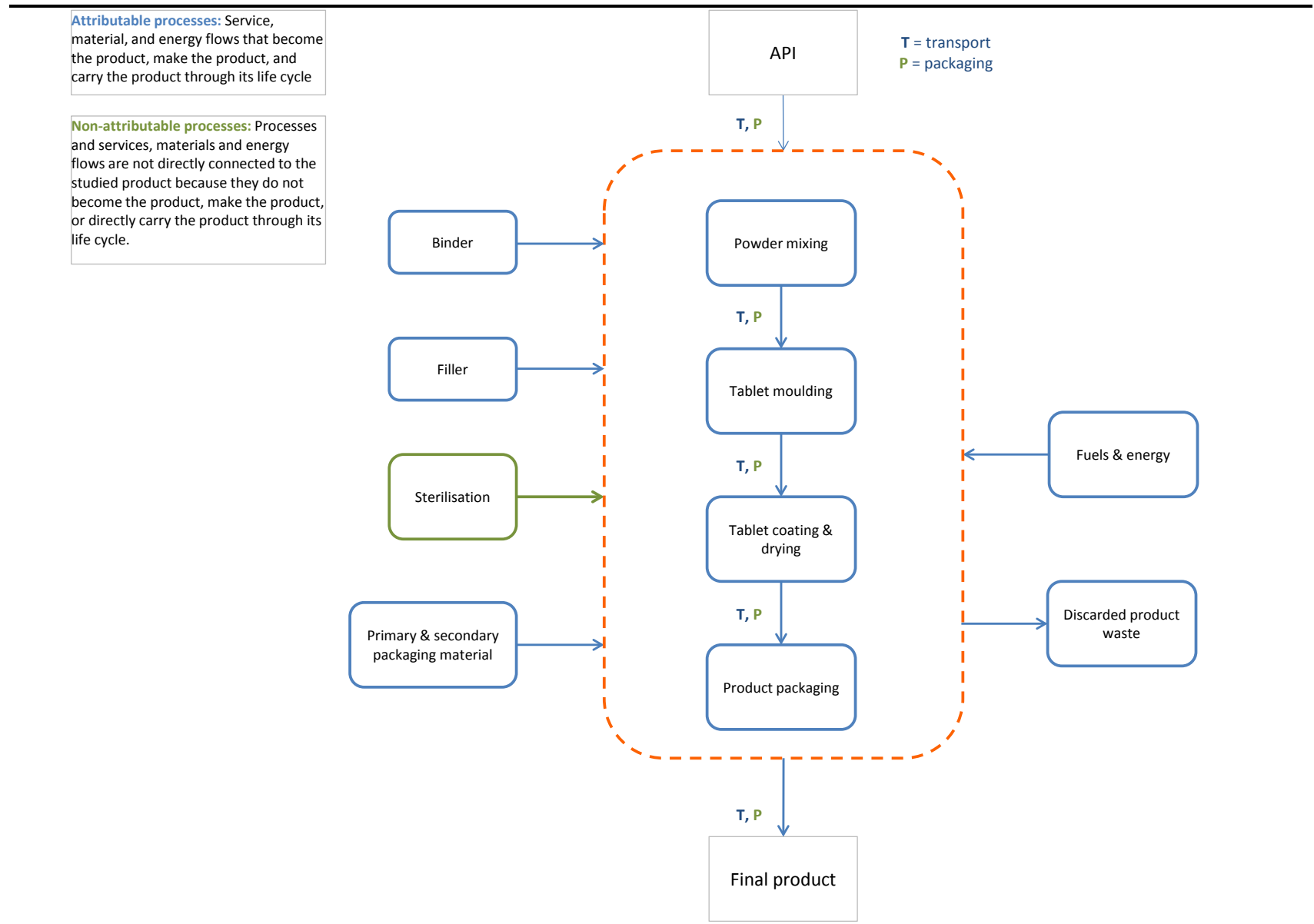
Figure 4.8 Sample Process Map for Solid Dose Forms (eg Tablets)
